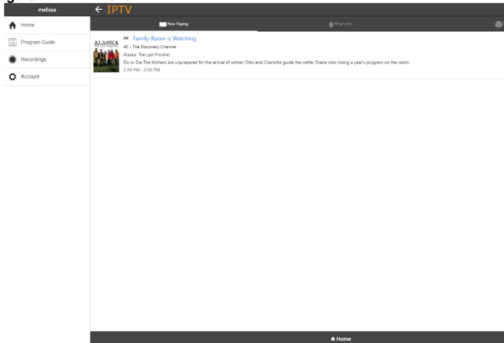
Figure 1-1 IPTV Menu
