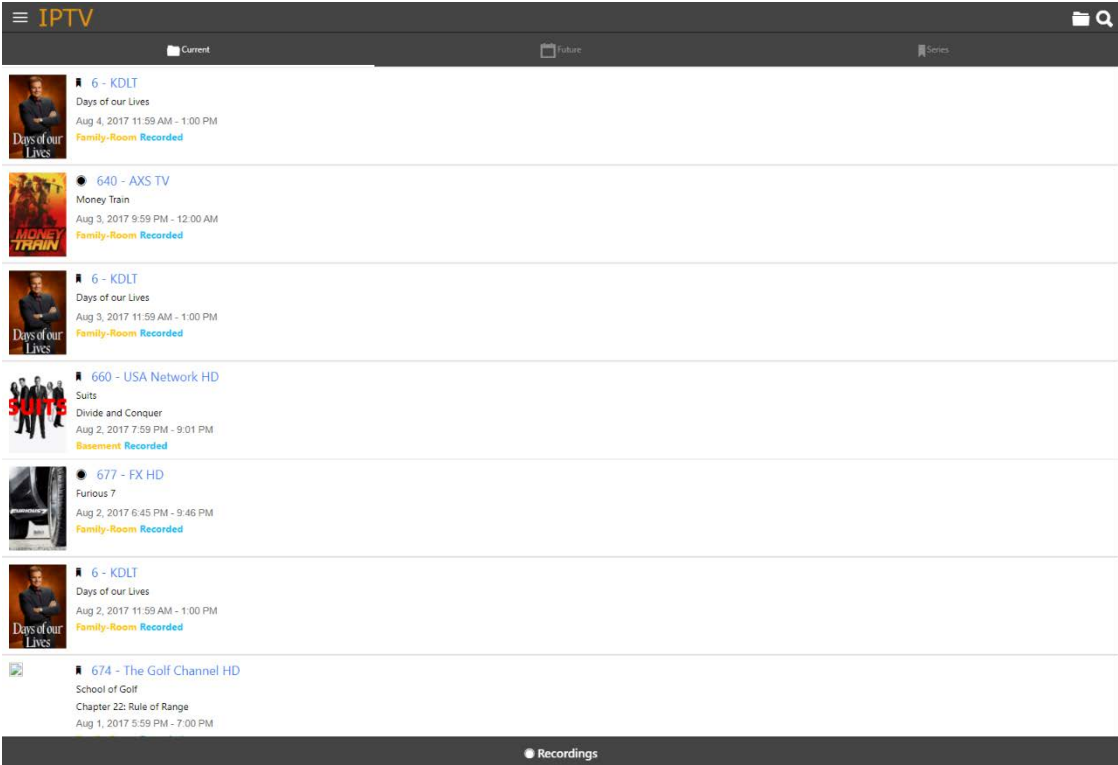
Figure 2-2 Recordings Tab
