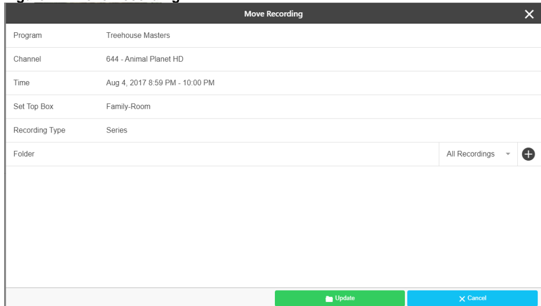
Figure 2-4 Move Recording
