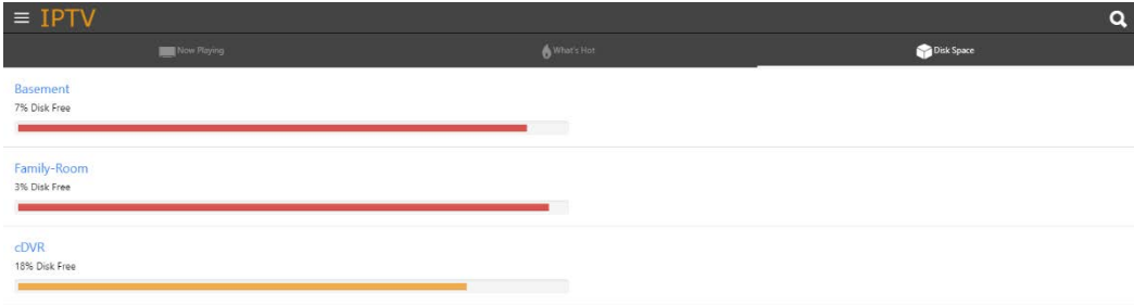
Figure 1-4 Disk Space
